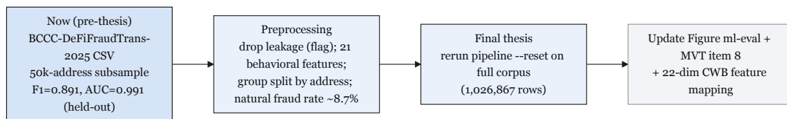
Figure 4.3: Dataset timeline
