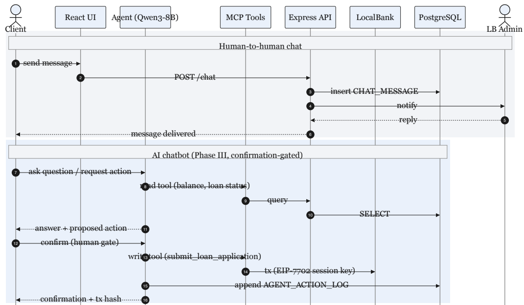
Figure 3.31: Sequence diagrams
