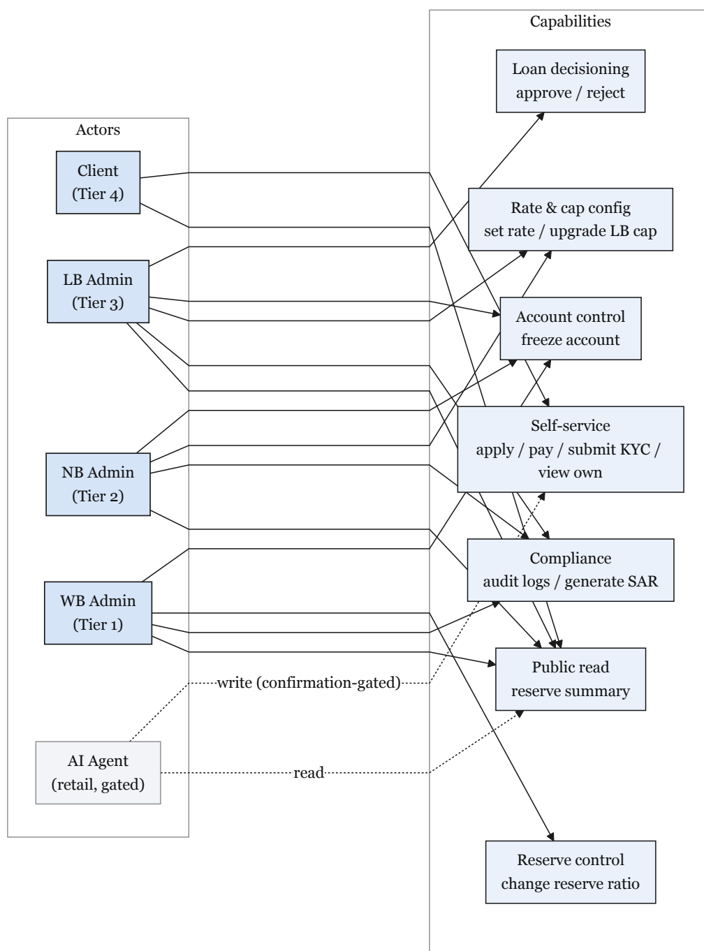
Figure 3.14: Actor permission matrix (primary actions)
