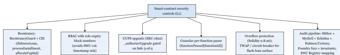
Figure 3.37: Smart-contract security controls
