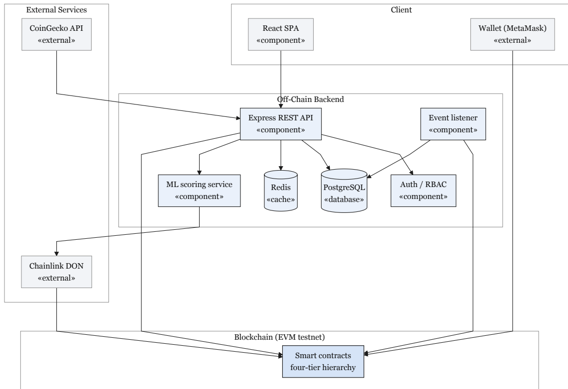
Figure 3.2: Component diagram (planning phase)
