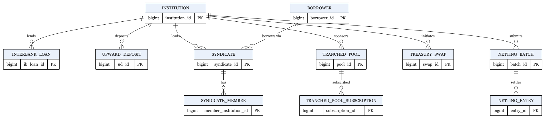
Figure 3.7: Extended ERD: multi-entity and cross-tier operational entities (crow's-foot; PK shown, full attributes in Table 3.14).
