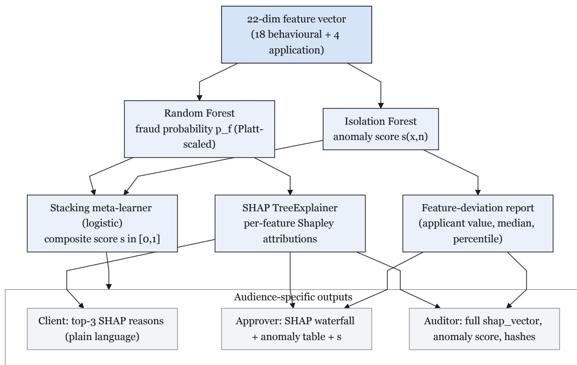
Figure 4.6: Explainability and anomaly-detection flow
