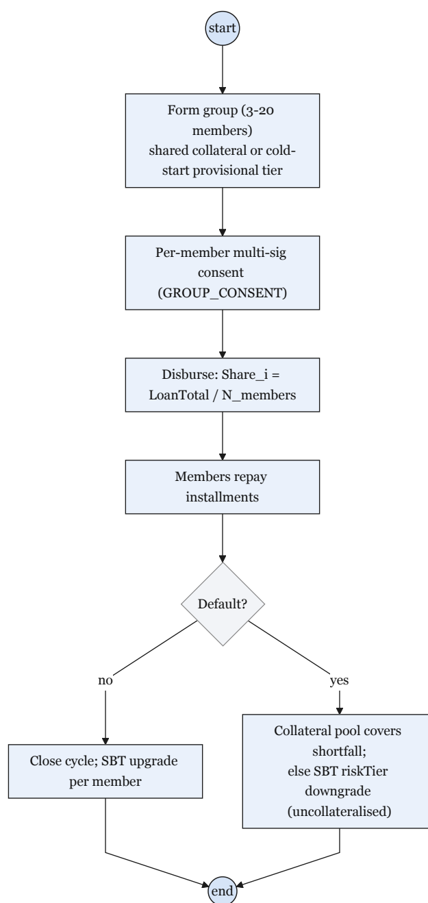
Figure 3.33: Solidarity group lending lifecycle
