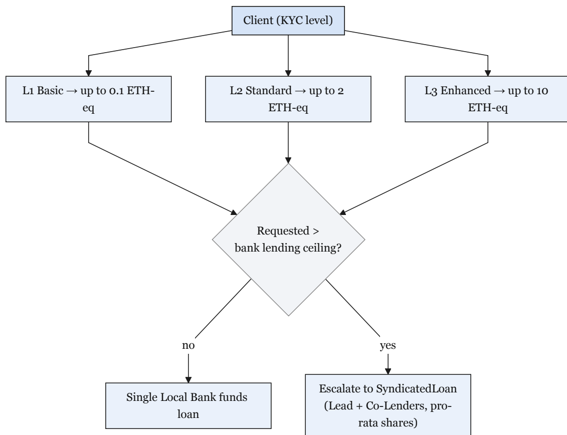
Figure 3.15: Client limits and bank-level syndication
