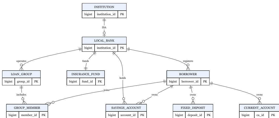
Figure 3.6: Extended ERD: banking-product entities (crow's-foot; PK shown, full attributes in Table 3.14).
