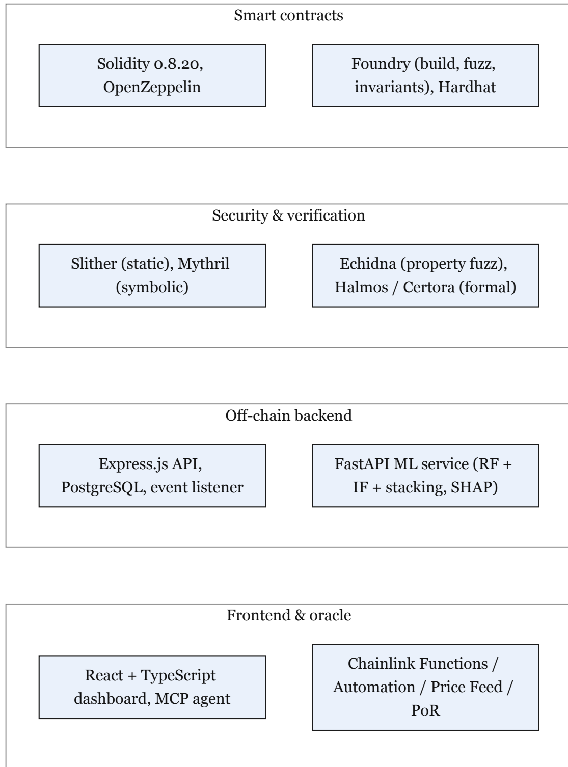
Figure 4.9: Planned development and verification toolchain
